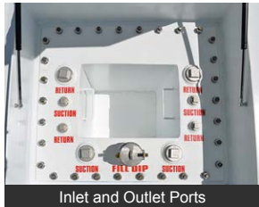
Inlet and Outlet Ports
